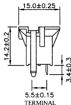
5.5±0.15 TERMINAL
