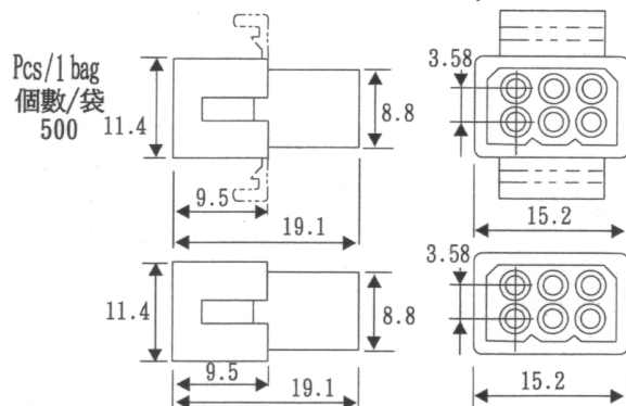
PART NO: H6656-09, 6656E-09
