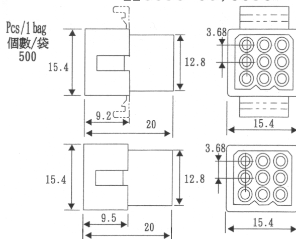
PART NO: H6656-09, 6656E-09
