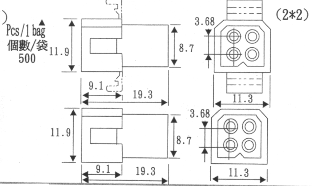
PART NO: H6656-05, 6656E-05
