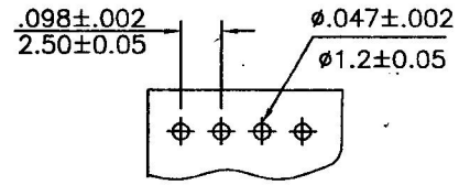
P.C. Board Layout
