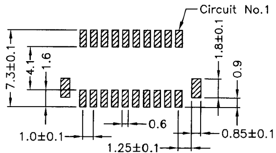
RECOMMENDED P. C. BOARD PATTERN DIM
